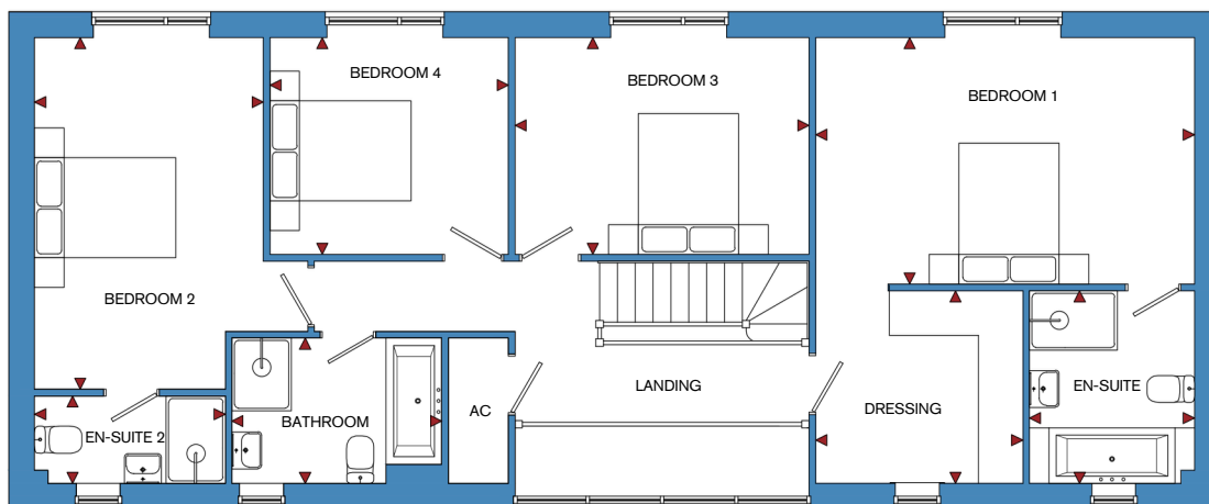
FIRST FLOOR
